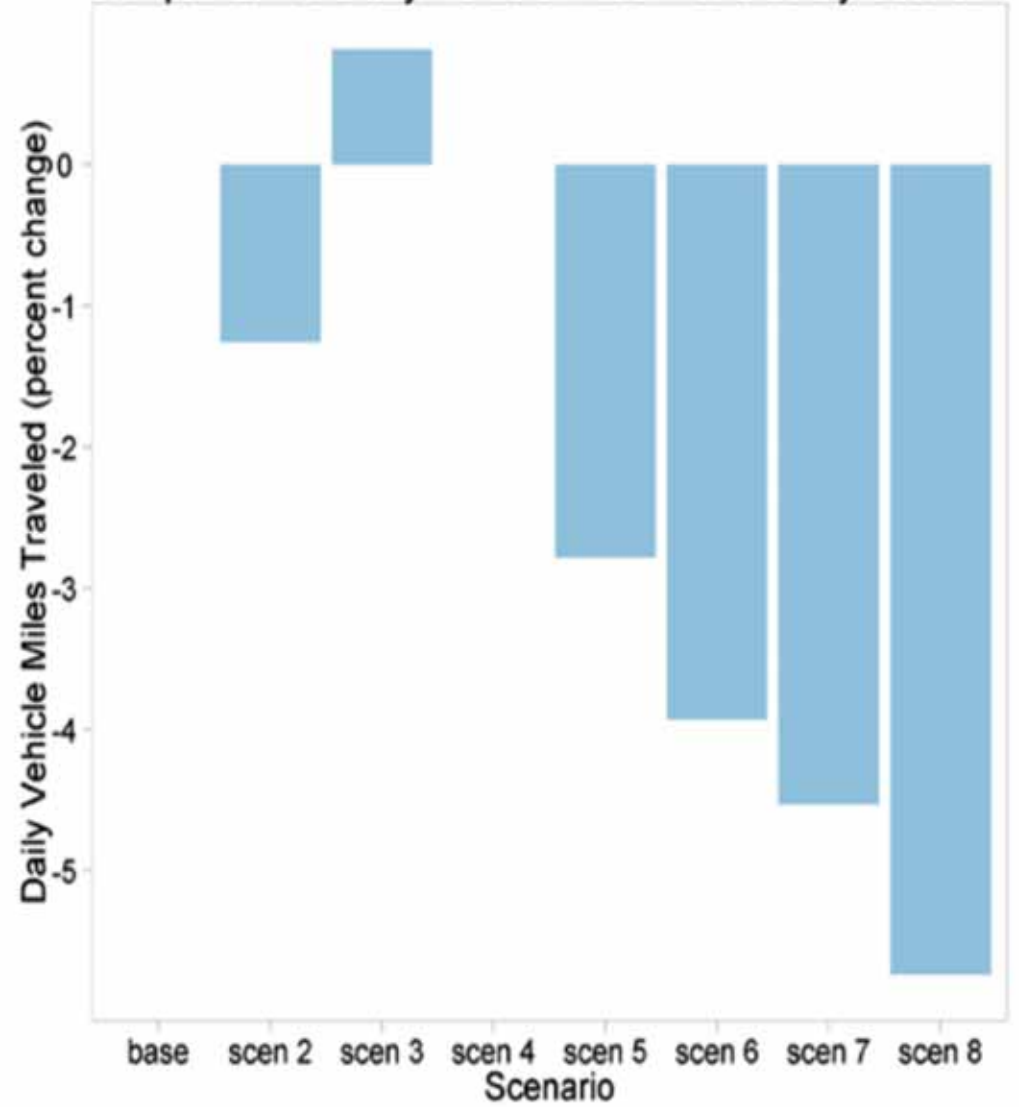
Comparison of Daily Vehicle Miles Traveled by Scenario
