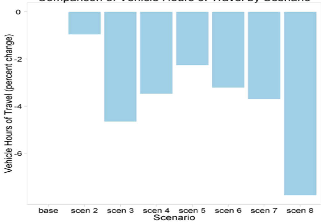
Comparison of Vehicle Hours of Travel by Scenario
